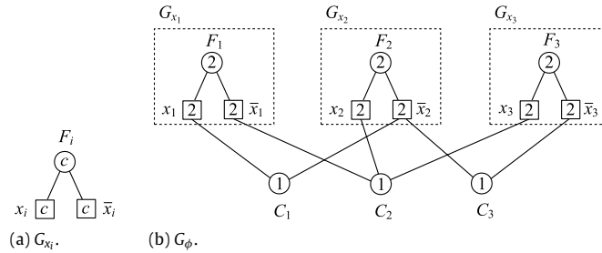
Fig. 2. (a) Variable gadget G_{x_i} , and (b) bipartite graph G_{\phi} corresponding to a Boolean formula \phi with three clauses C_1 = (x_1 \vee \bar{x}_2) , C_2 = (\bar{x}_1 \vee x_2 \vee x_3) and C_3 = (\bar{x}_2 \vee \bar{x}_3) , and hence c = 2 .
