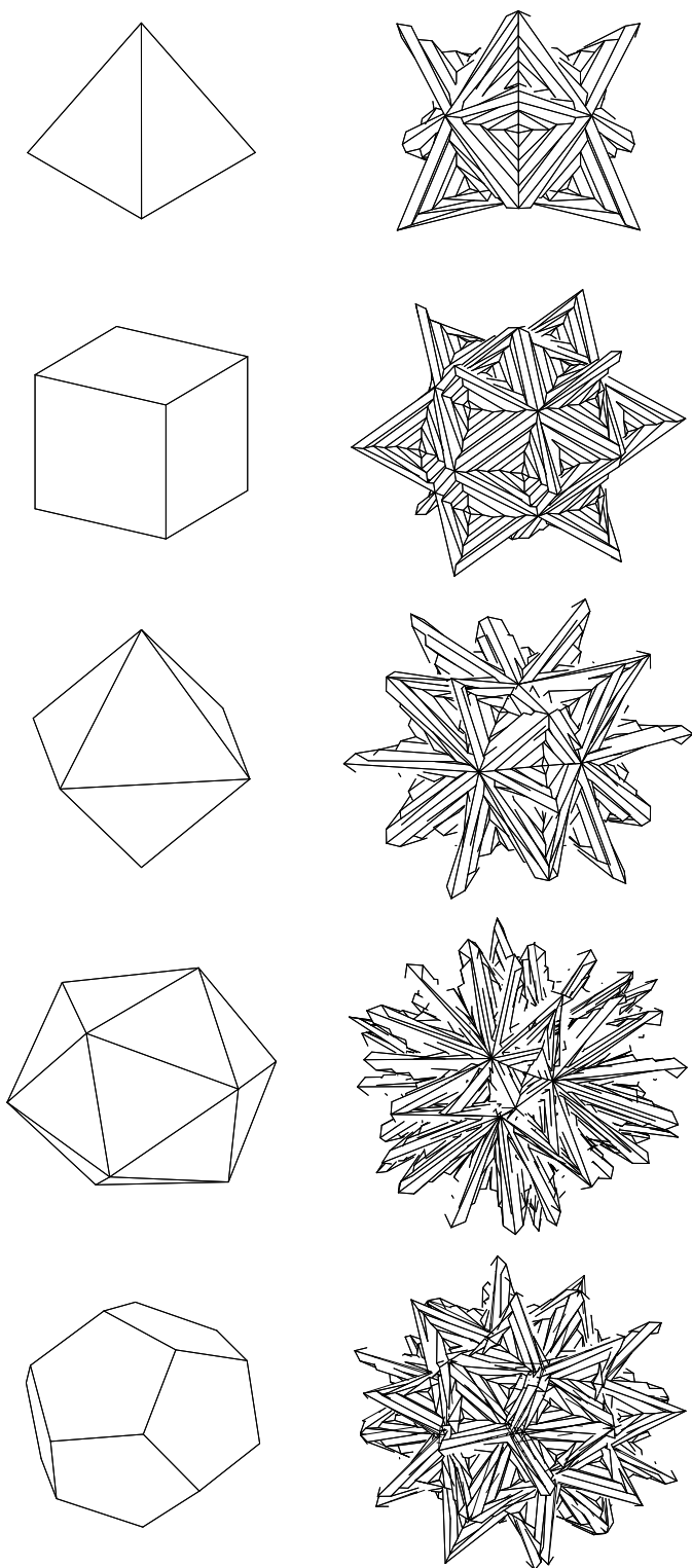
Figure 6: The Platonic solids and corresponding hyperhedra (computer and physical models). The view angles are the same for the left two columns, except for the tetrahedron. The physical models were constructed from six-inch squares of paper, and take 2–6 hours each to construct.
