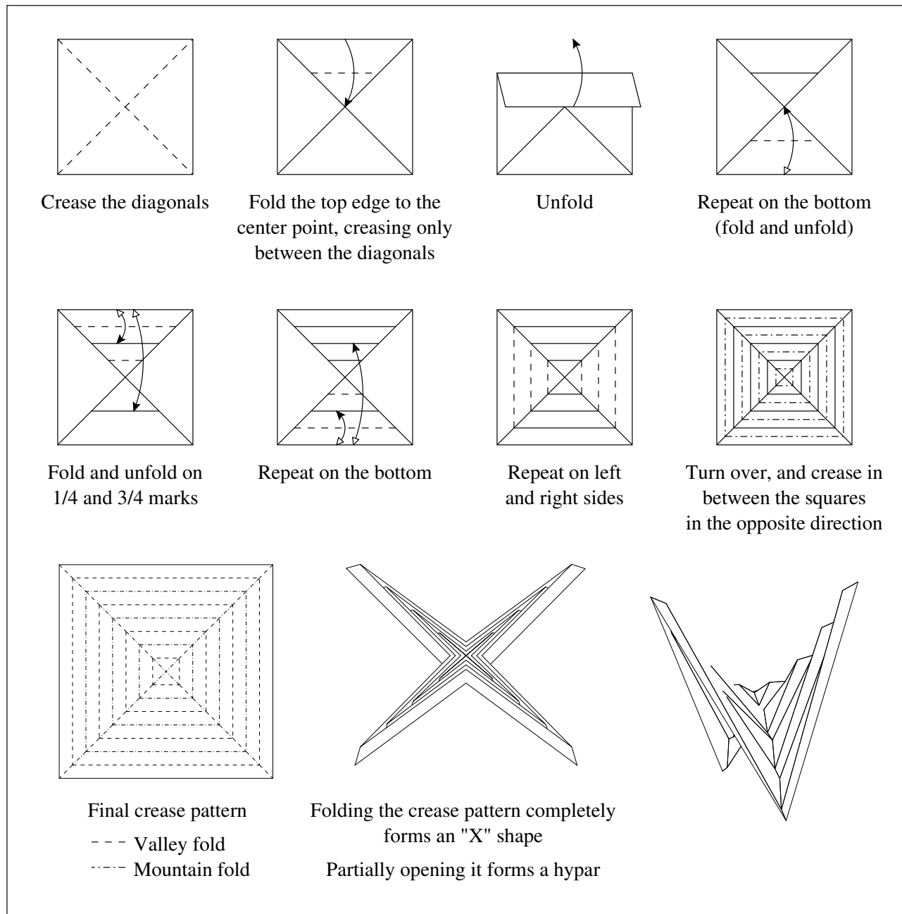
Figure 2: Folding a hyper from a square.
