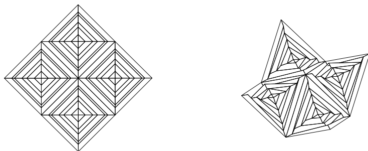
Figure 5: A 4-hat from overhead and side views.
