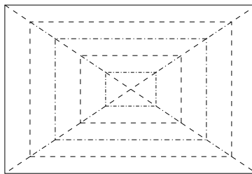
Figure 4: A different hypar folding from a rectangle.
