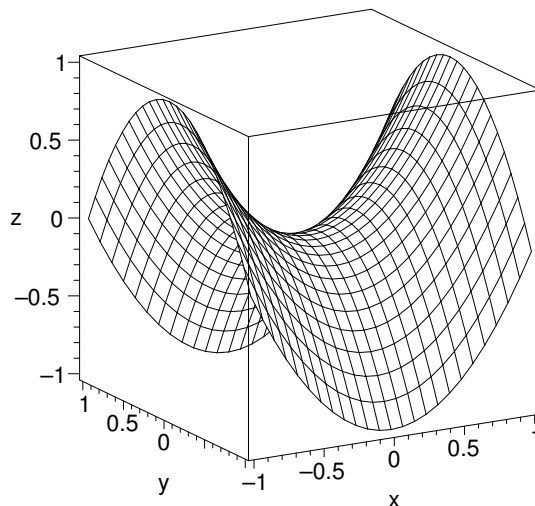
Figure 1: A hyperbolic paraboloid z = x^2 - y^2 .
